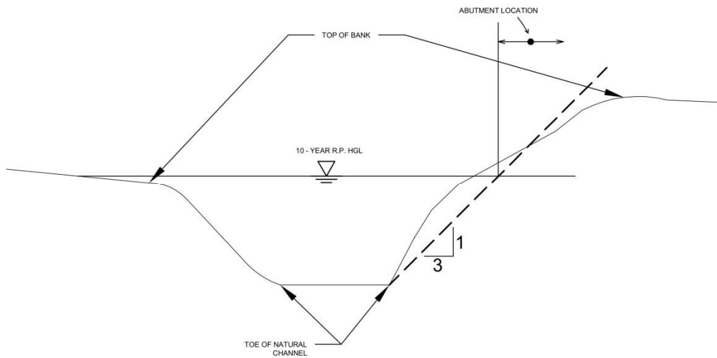
Case 2 - Steep and High Bank
