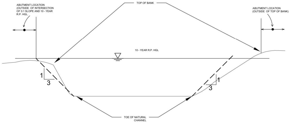
Case 1 - Steep and Flat Banks
